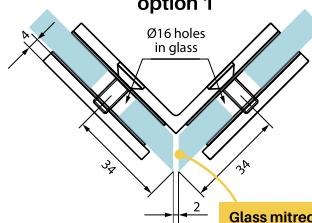
Glass configuration option 1
