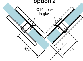
Glass configuration option 2
