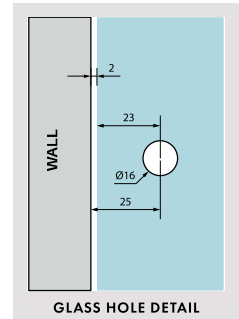
GLASS HOLE DETAIL
