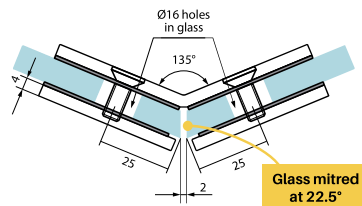
Glass configuration
