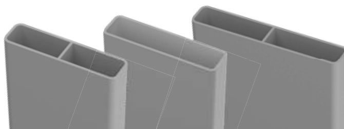
65mm x 16.5mm slat with centre web
