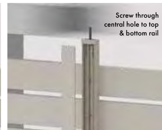
Screw top/bottom plate to centre support rail
