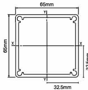
65x65mm heavy duty post 2400MM or 6000MM LONG Order Code: XP-2400/6000-65HD
